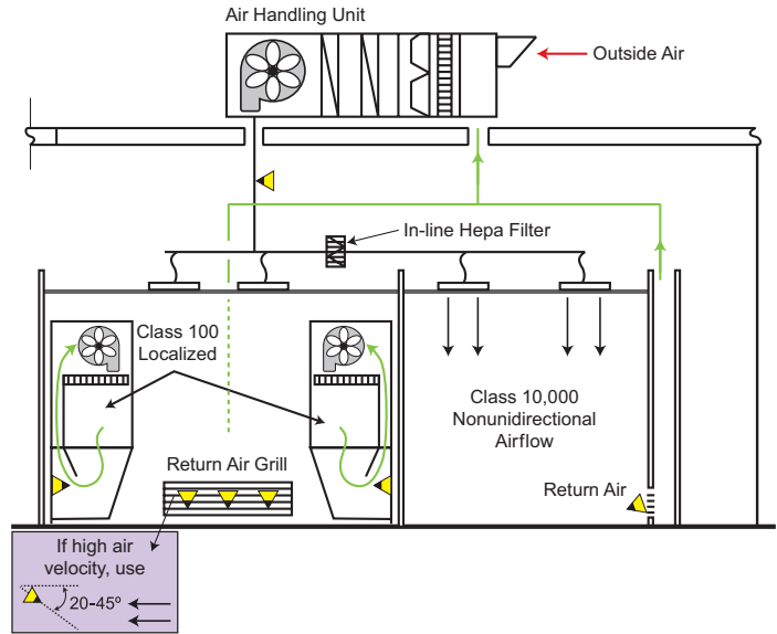
Concepts for air flow path smoke detection in a cleanroom scenario. Shown are primary air sample point locations:
