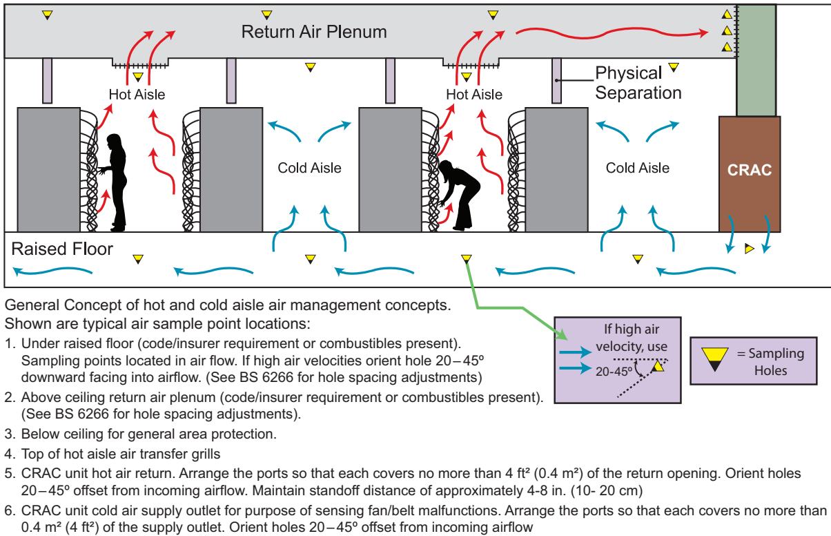
Figure 9 – General Concept of Hot and Cold Aisle Air Management in Data Centers
