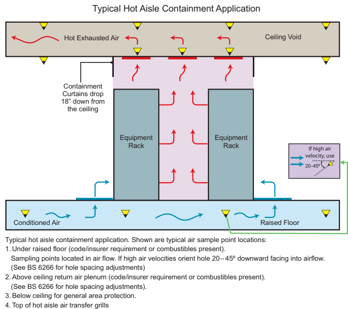
Figure 10 - Hot Aisle Containment application
