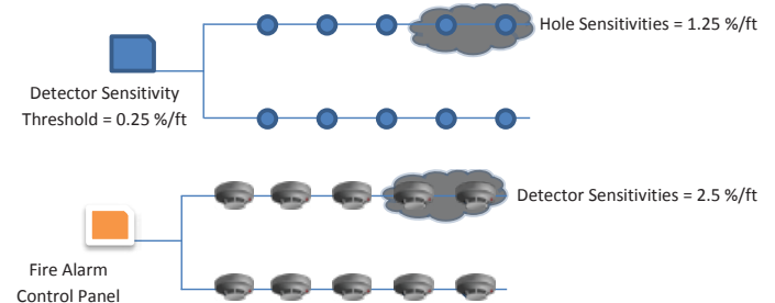
Figure 9. Comparison (ASD – point smoke detector) with smoke reaching two sampling holes or two spot smoke detectors
