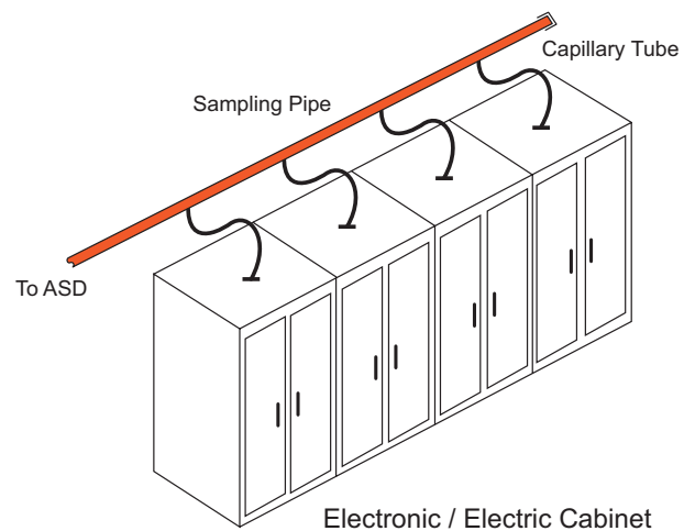
Figure 7. Sampling electronic / electrical cabinets utilizing capillary sampling points
