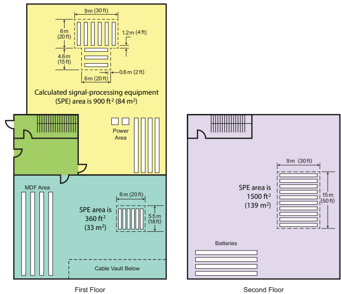
The first floor considered alone would not exceed the 2500 ft 2 (232 m 2 ) threshold as the combined SPE area is 1260 ft 2 (117 m 2 ). Adding a second story increases the aggregate SPE area to 2760 ft 2 (256 m 2 ).
