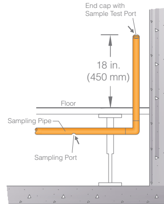
Figure 10. 3-Test sample point for void space or subfloor
