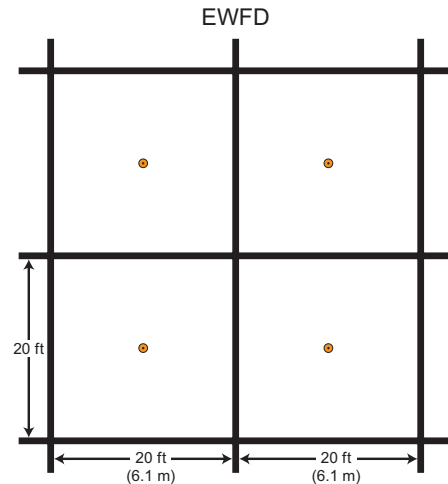
Example arrangement of sampling ports located to meet requirements for EWFD in structural bays of 400 ft 2 (37.2 m 2 )
