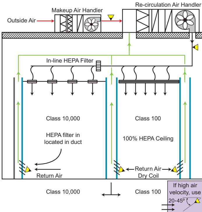
Concepts for air flow path smoke detection in a cleanroom scenario. Shown are primary air sample point locations:
