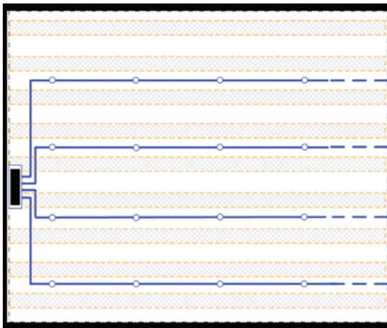
Figure 16 – Sampling pipe layout for storage rack area, where racks stop well below the ceiling (non-branched pipes parallel to rack orientation)
