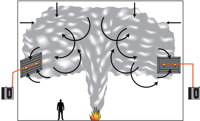
Scenario 6: Forced ventilation systems serving large volume spaces can result in turbulent, well-mixed air flow conditions. Small, moderate and large fire plumes can be interrupted and diluted by these normal air flows. A potentially effective method to provide for smoke detection is to provide aspirating sampling points to capture diffuse and diluted smoke at ventilation system air returns. In situations where the ventilation is modulated or turned off ceiling detection sampling points may also need to be provided to assure detection when forced ventilation is low.
