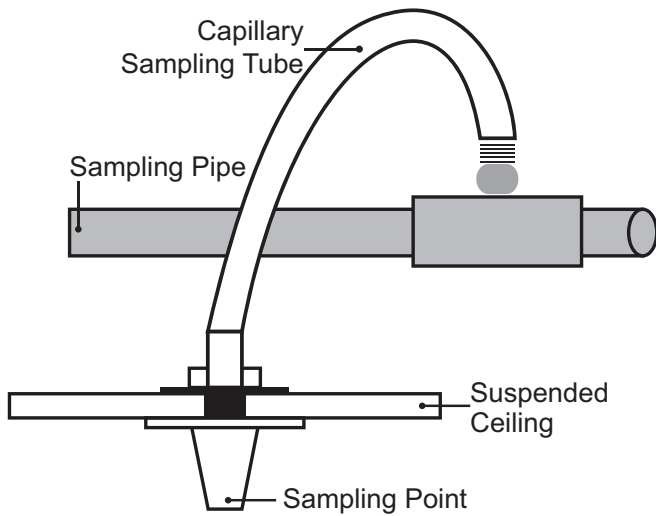
Figure 5. Capillary used for an ASD sampling pipe network
