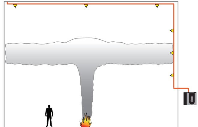
Scenario 4: Where the objective is to detect fires when they are relatively small with limited smoke buoyancy or where temperature changes in the space may cause stratification the use of sampling points at multiple elevations can be an effective aspirating detection solution. In many cases, ceiling detection sampling points should also be provided to assure detection of larger buoyant fire plumes that will push smoke readily to the ceiling.
