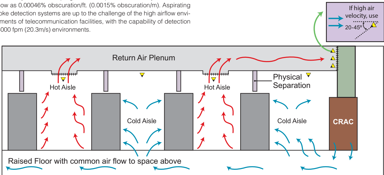
General Concept of telecommunications SPE area using hot and cold aisle air management concepts. Shown are typical air sample point locations.
