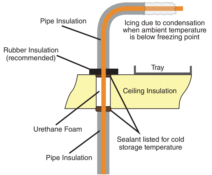
Figure 8. Ceiling insulating pipe
