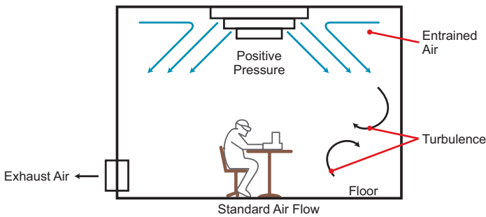
Figure 5. Standard airflow within a conventional cleanroom
