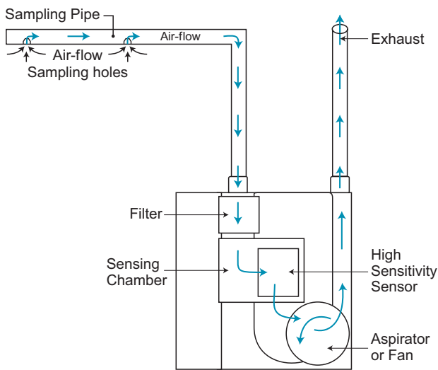
Figure 1. Basic aspirating smoke detection system The blue arrows illustrate the air flow from the time it enters the sampling pipe to the point it is exhausted out of the ASD.
