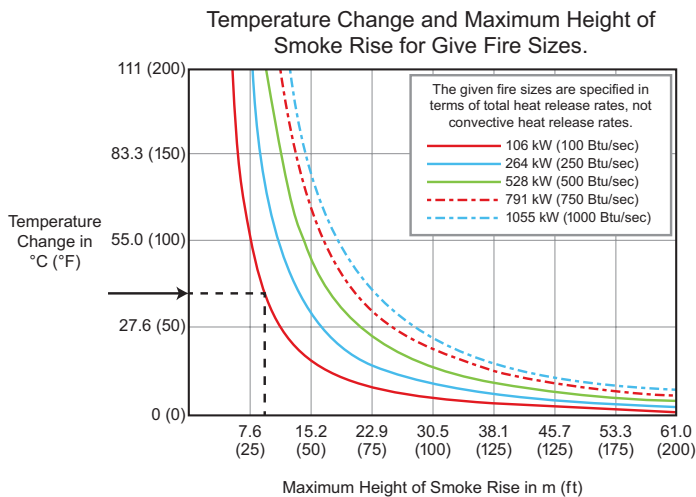
Figure 12 – Smoke Rise in Spaces with a Uniform Temperature Gradient
