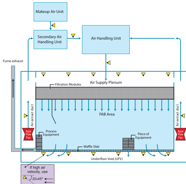
Concept of aspirating smoke detection in semiconductor fabrication facilities. Shown are typical required smoke detection locations (make-up and air handling units) and various options for providing smoke detection in the clean room return airstream at locations before dilution with make-up air occurs. One or more of the following locations are recommended (see NFPA 318, Annex A) when using aspirating smoke detection:
