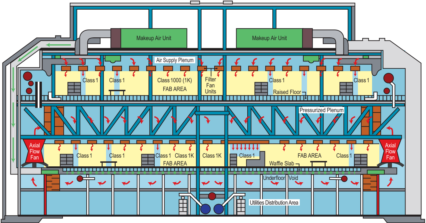
Areas of a large semiconductor facility and the many airflow paths that exist.
