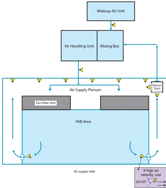
Concept of aspirating smoke detection in semiconductor fabrication facilities. Shown are typical required smoke detection locations (make-up and air handling units) and various options for providing smoke detection in the clean room return airstream at locations before dilution with make-up air occurs. One or more of the following locations are recommended (see NFPA 318, Annex A) when using aspirating smoke detection:
