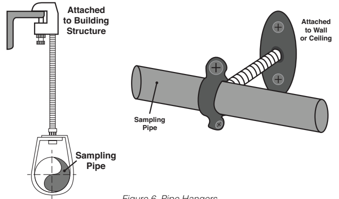
Figure 6. Pipe Hangers
