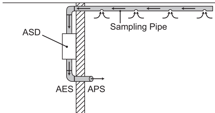
Figure 6. ASD Exhaust – AES vs APS
