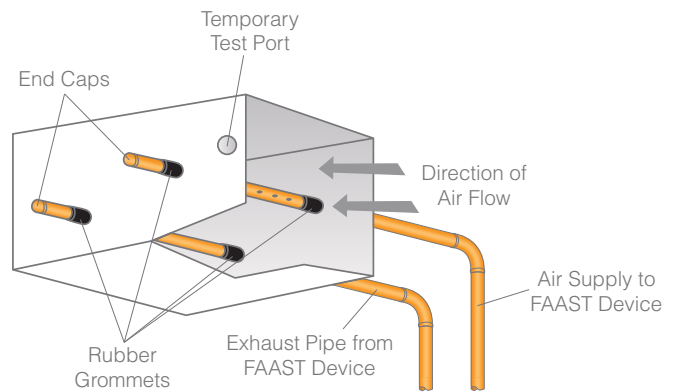
Figure 1. Design consideration for in-duct sampling
