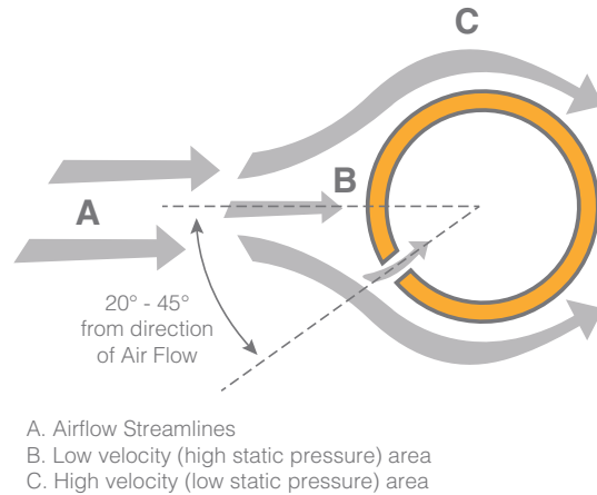
Figure 7. Sampling hole orientation
