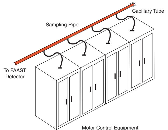
Figure 5. Sampling motor control units utilizing capillary sampling points
