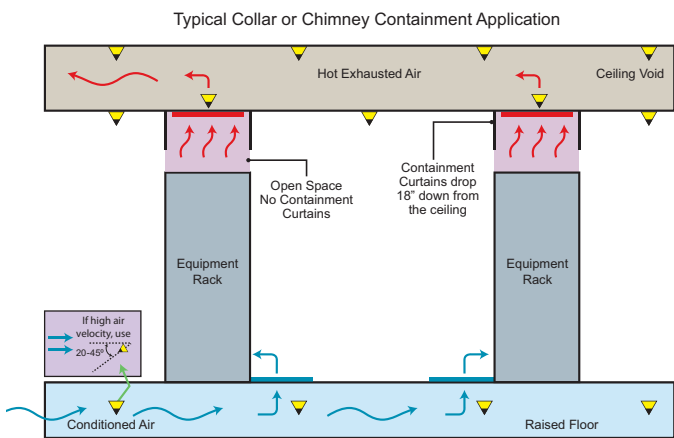
Figure 11 – Cold Aisle Containment application
