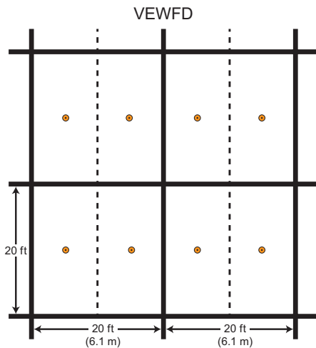
Example arrangement of sampling ports located to meet requirements for VEWFD in structural bays of 400 ft 2 (37.2 m 2 )
