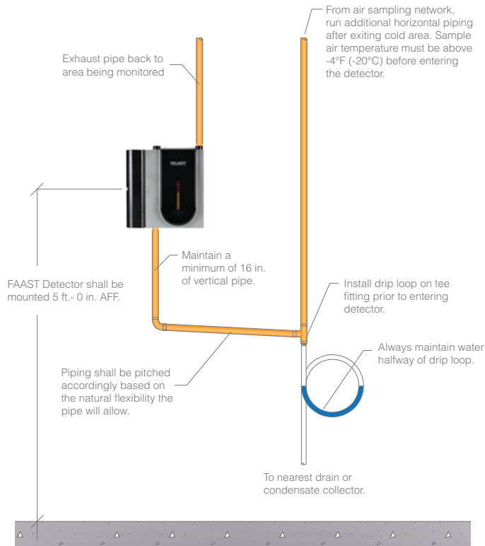
Figure 2. Drip loop installed in sampling pipe
