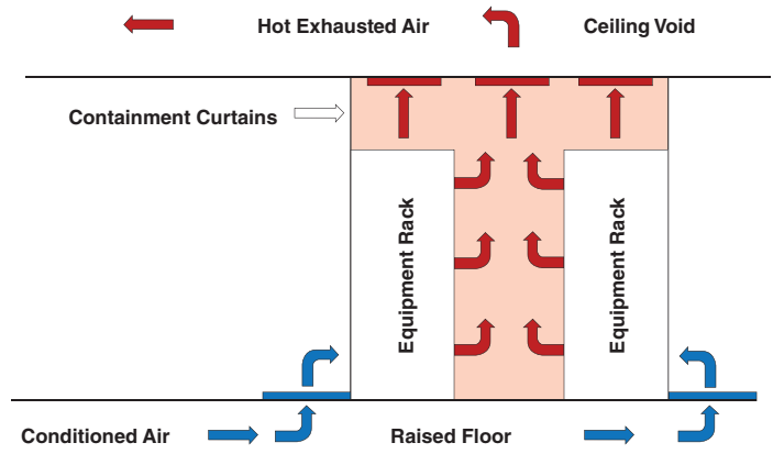
Figure 12. Typical hot air aisle containment configuration
