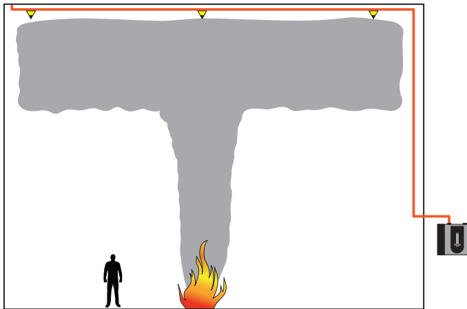
Scenario 1: Where the hazard to be detected concerns growing fires with well-developed fire plumes locating aspirating sampling points on the high ceiling is appropriate for this case of detecting large or growing fires. In large volume spaces the ceiling sampling points can provide detection long before the smoke hazard will descend to the occupied areas.
