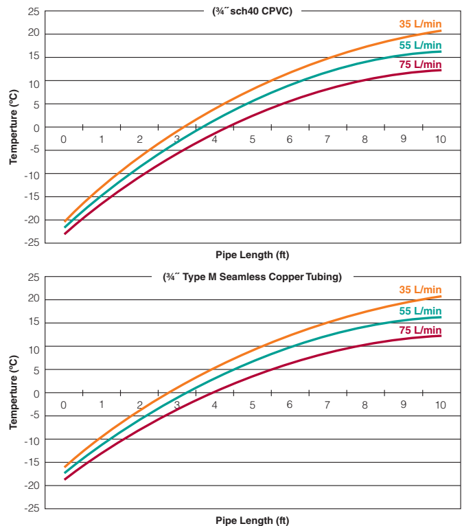
Figure 6. Distances needed to heat air in sampling pipe
