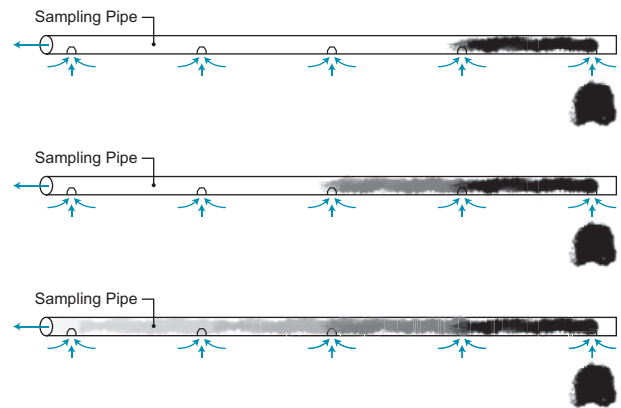
Figure 7. The Dilution Effect
