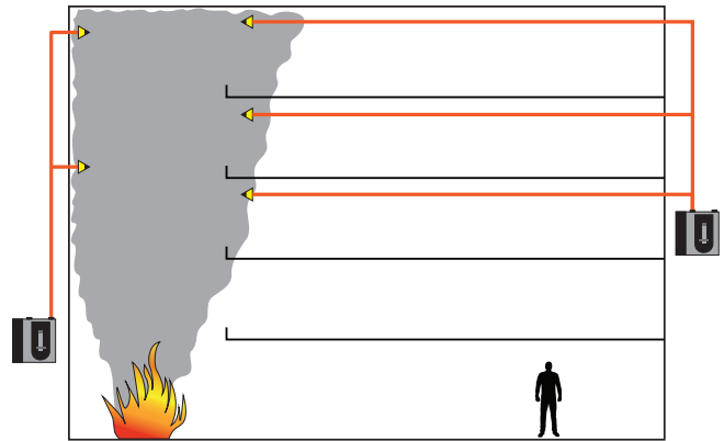
Scenario 3: Where the hazard to be detected concerns growing fires with well-developed fire plumes that spill into a tall narrow space. In this case a fire plume can be expected to contact the side walls. This occurs when the distance across the narrow space equals approximately 40% of the height of the rising fire plume. For example a fire plume (centered in the space) that rises 50 ft. will contact the side walls of a space that is 20 feet wide. In this situation air sampling points located only on the side walls or perimeter floor areas of the tall narrow space can be sufficient to capture and detect smoke filling the space.
