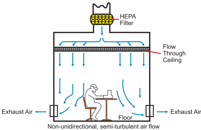
Figure 6. Semi-laminar airflow within a Class 10,000 cleanroom
