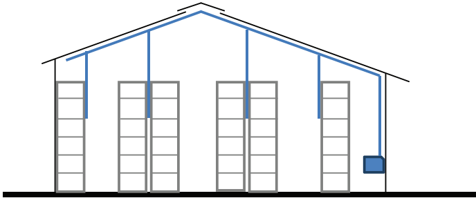
Figure 19. Example of drop-down pipes for in-rack ASD
