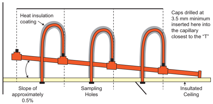
Figure 9. Capillary installation methods in cold storage
