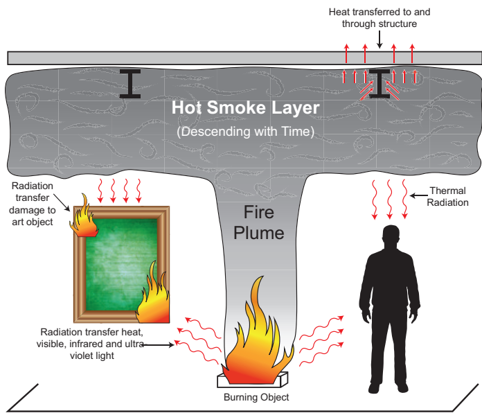
Figure 4 – Fire Environment in a Heritage Environment
